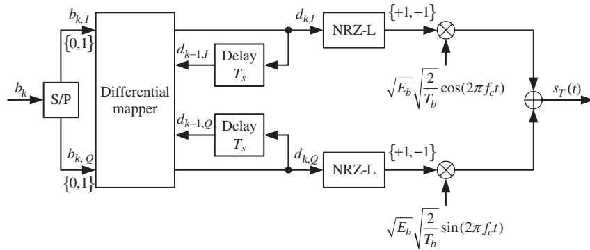
Fig. 10.23 Block diagram of the modulator for DQPSK.
