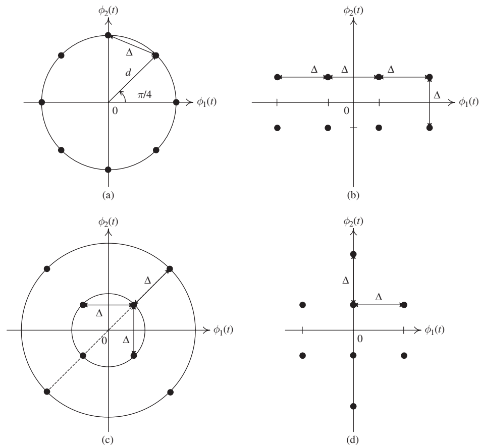
Fig. 8.28 The 8-ary constellations considered in Problem 8.9.
