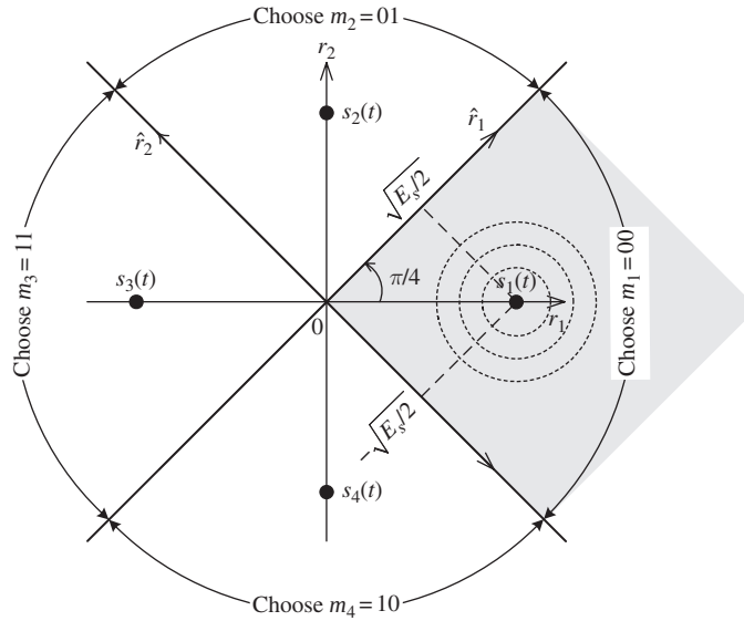
Fig. 7.14 Signal space diagram of QPSK: to compute P[\text{correct}|s_1(t)] one finds the volume of f(\hat{r}_1, \hat{r}_2 | s_1(t)) over the shaded quadrant.
