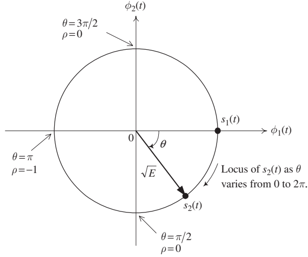
Fig. 5.12 Signal space representation for signal set in Example 5.5.
