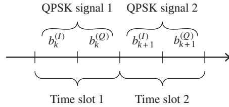
Fig. 11.51 Transmission of two consecutive QPSK symbols.
