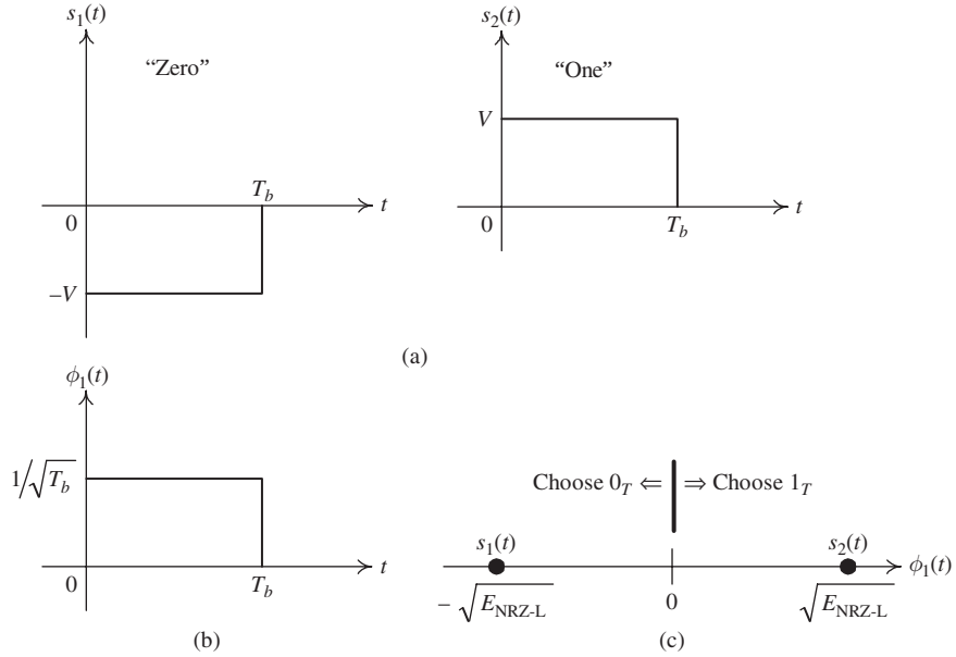
Fig. 6.5 NRZ-L code: (a) elementary signals; (b) basis function; (c) signal space and decision regions.
