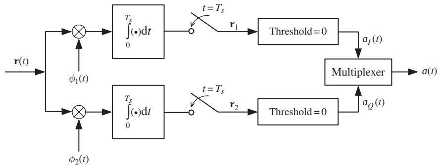
Fig. 7.20 Receiver implementation for QPSK.
