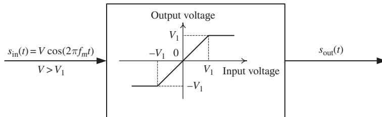
Fig. 2.32 Illustration of signal clipping.
