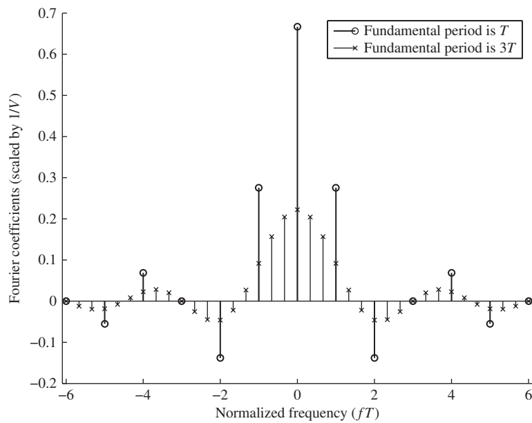
Fig. 2.17 Illustration of the effect of increasing the fundamental period while keeping the basic pulse p(t) unchanged. Here p(t) is a rectangular of amplitude V over [-T/3, T/3] .
