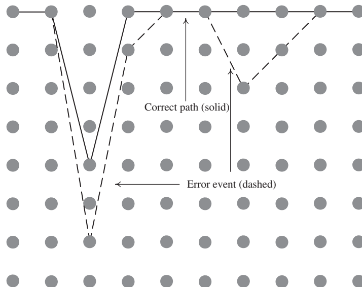
Fig. 11.21 Illustration of an error event.
