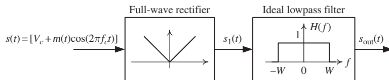
Fig. 2.40 Block diagram of envelope detection of amplitude modulation.
