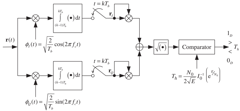
Fig. 10.5 Block diagram of the optimum receiver for BASK under random phase.
