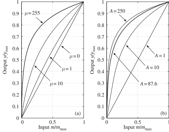
Fig. 4.12 Compression characteristic: (a) \mu -law and (b) A -law. Note that both characteristics are odd functions and only the positive half of the input signal is illustrated.
