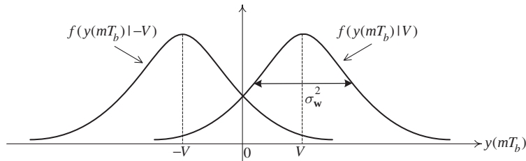
Fig. 9.15 The conditional pdfs of \mathbf{y}(mT_b) .
