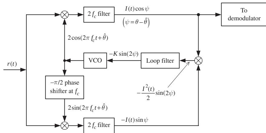
Fig. 12.17 Costas loop for carrier recovery for BPSK.
