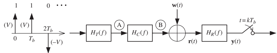
Fig. 9.2 Impulse modulator.
