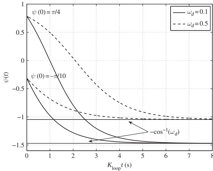
Fig. 12.9 Plots of \psi(t) for different values of \omega_d and \psi(0) .
