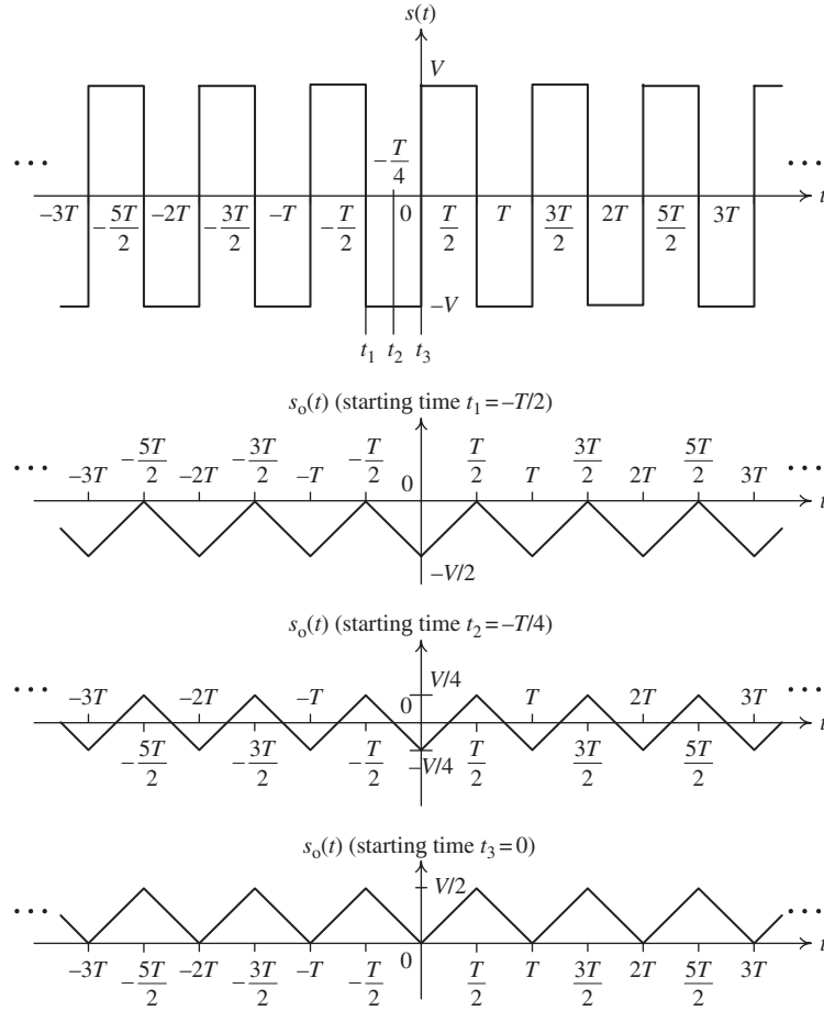
Fig. 2.9 Effect on output signal of different starting times for the integrator.
