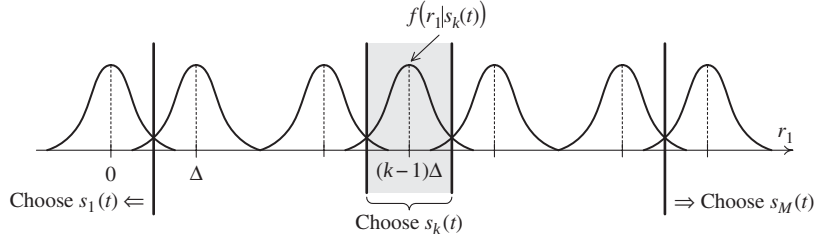
Fig. 8.5 Decision regions for M -ASK.
