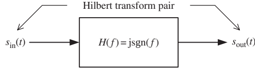
Fig. 2.43 The LTI system considered in Problem 2.50.
