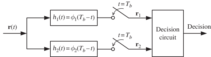
Fig. 5.17 Receiver implementation using matched filters.
