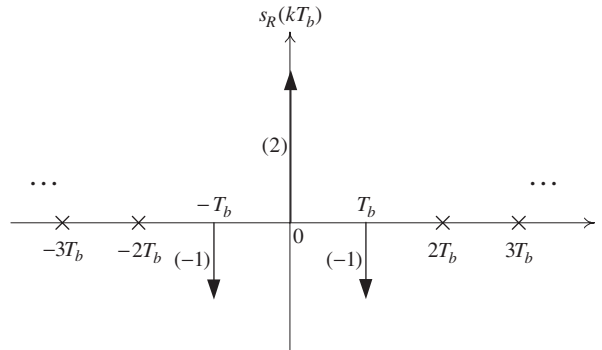
Fig. 9.37 The sampled overall impulse response considered in Problem 9.13.
