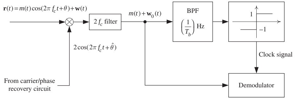
Fig. 12.19 Clock recovery circuit when m(t) has a spectral component at 1/T_b hertz. Here BPF means bandpass filter.
