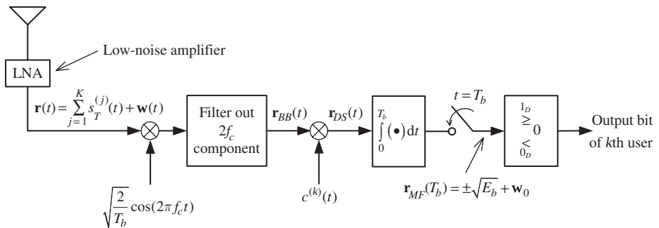
Fig. 11.36 CDMA demodulator for the k th user.
