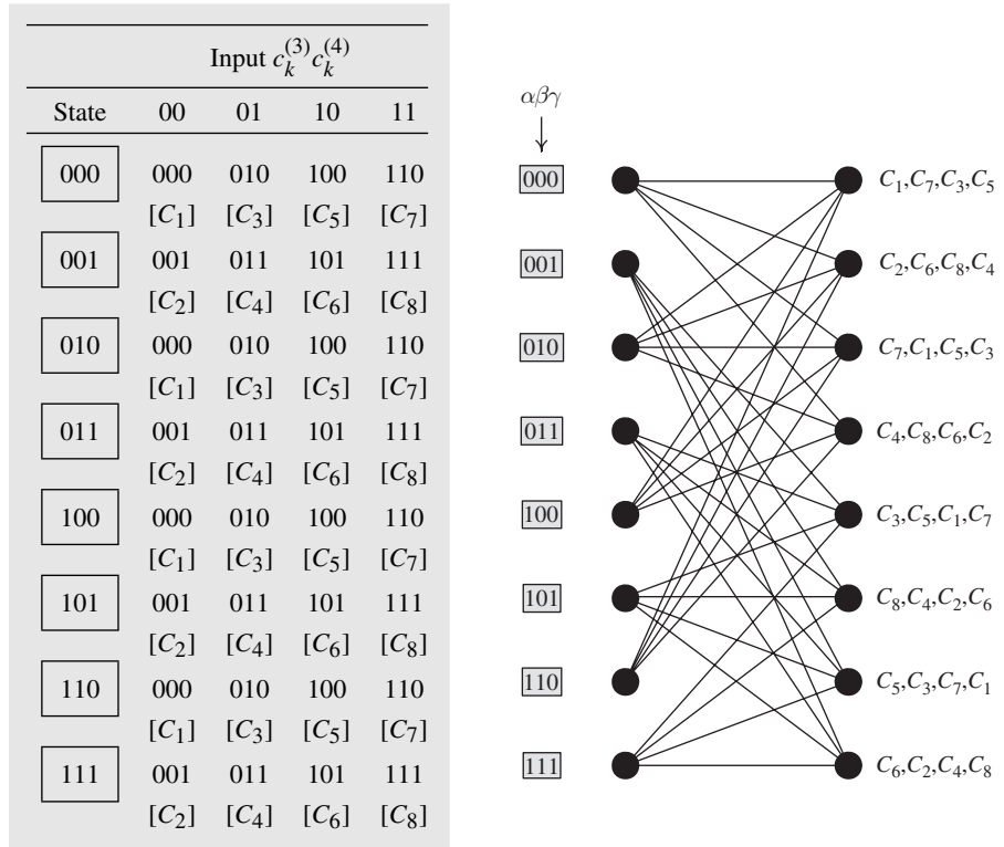
Fig. 11.28 Trellis diagram of V.32 differential TCM. The table on the left shows the “coded” bits c_k^{(3)} c_k^{(4)} used to select the coset, which is written in the squared brackets underneath.
