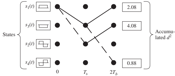
Fig. 6.16 Distances squared of the survivor paths after the second bit interval.
