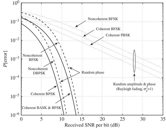
Fig. 10.16 Error performance of noncoherent and coherent BFSK and coherent BPSK over a Rayleigh fading channel.
