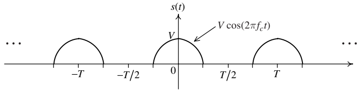
Fig. 2.31 Output of a half-wave rectifier.
