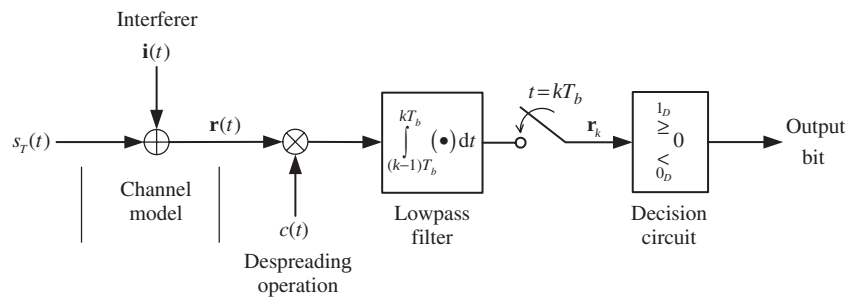
Fig. 11.31 Spread spectrum receiver.
