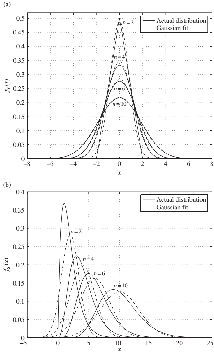
Fig. 10.20 Illustration of the central limit theorem: (a) i.i.d. uniform random variables; (b) i.i.d. Laplacian random variables.
