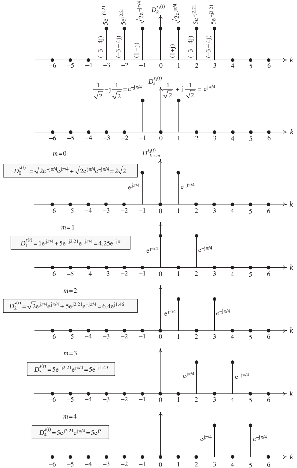
Fig. 2.15 Fourier coefficients of the product of two periodic signals determined by graphical convolution.
