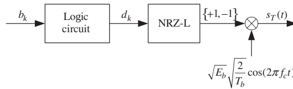
Fig. 10.22 Block diagram of the modulator for DBPSK.
