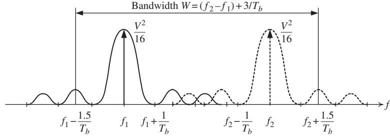
Fig. 7.7 Bandwidth approximation for BFSK.
