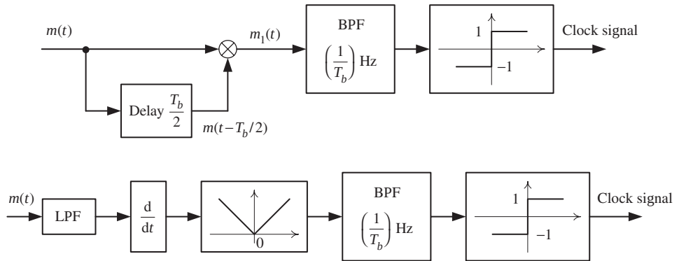
Fig. 12.20 Two different open-loop symbol synchronizers in which the baseband modulation has no spectral component at 1/T_b hertz. Note that, for clarity, noise component w_0(t) is ignored. Also LPF means lowpass filter.
