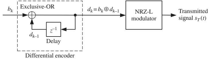
Fig. 6.21 Differential NRZ-L modulation.
