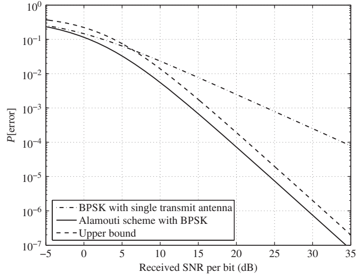
Fig. 11.50 Bit error probability of the Alamouti scheme with BPSK. Also shown for comparison are its upper bound and the bit error probability of BPSK with one transmit and one receive antennas.
