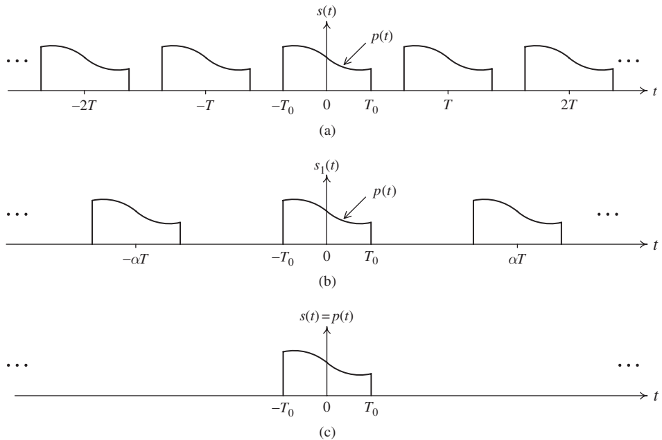
Fig. 2.16 Derivation of the Fourier transform of a nonperiodic signal: fundamental period is (a) T , (b) \alpha T, \alpha > 1 , (c) approaching \infty .
