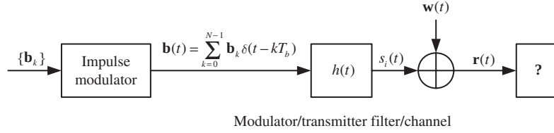
Fig. 9.22 System block diagram.
