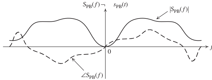
Fig. 2.44 Illustration of the magnitude and phase spectra of a passband signal.
