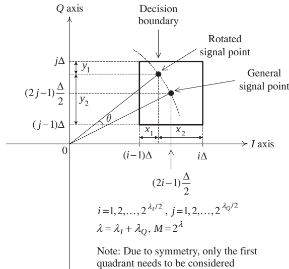
Fig. 12.23 Geometrical representation of a general QAM signal point with phase uncertainty.
