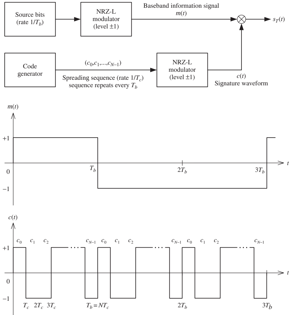
Fig. 11.30 Spread spectrum transmitter.
