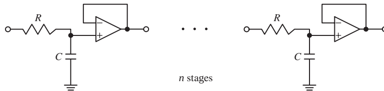
Fig. 10.21 A cascade of n identical lowpass filters.
