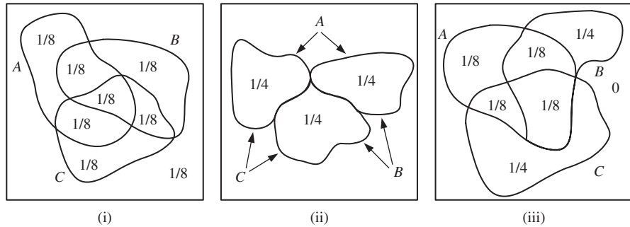
Fig. 3.23 Three Venn diagrams considered in Problem 3.11.
