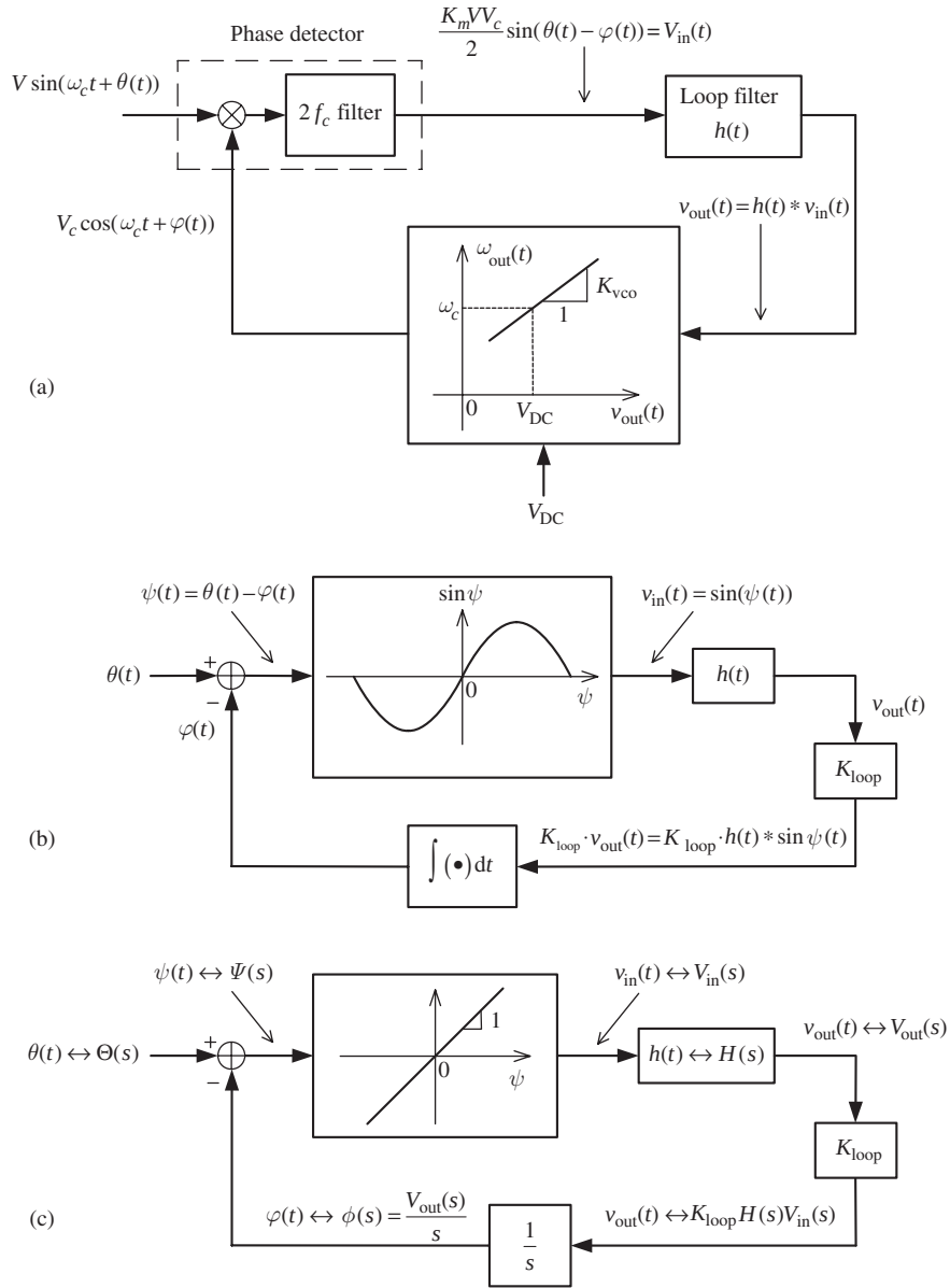
Fig. 12.10 PLL models: (a) sinusoidal PLL, (b) equivalent model of the sinusoidal PLL, (c) linear model of the sinusoidal PLL.
