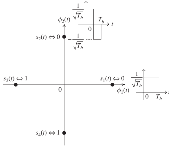
Fig. 6.24 Signal space diagram of Class2K modulation.
