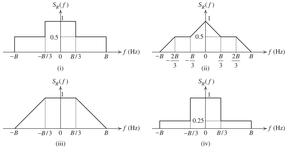
Fig. 9.35 The four overall system responses considered in Problem 9.8.
