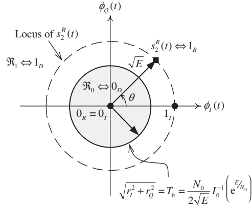
Fig. 10.4 Decision regions of BASK with random phase.
