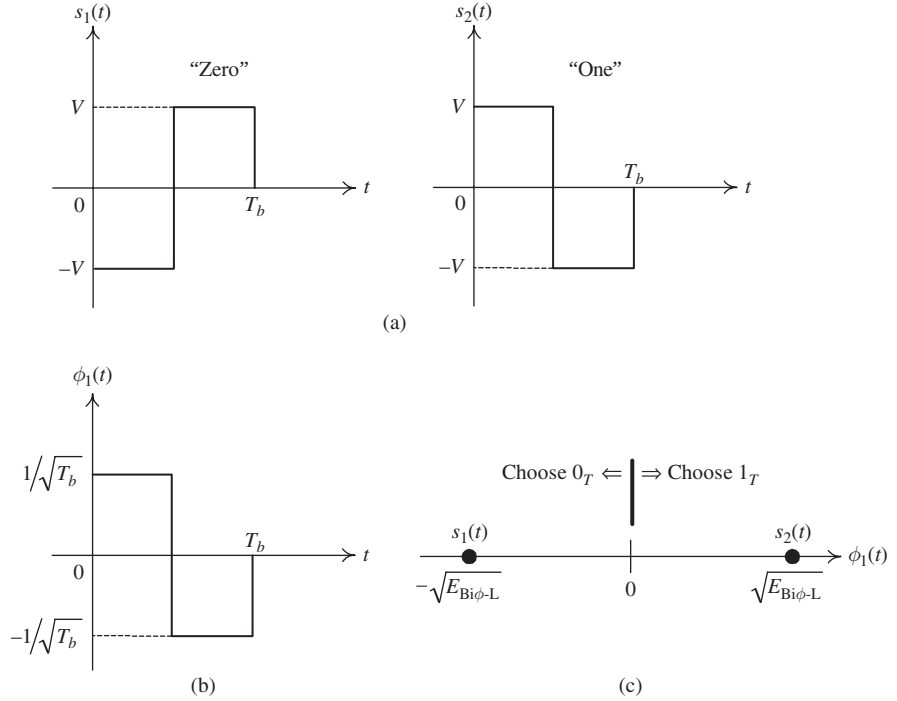
Fig. 6.7 Biφ-L code: (a) elementary signals; (b) basis function; (c) signal space and decision regions.
